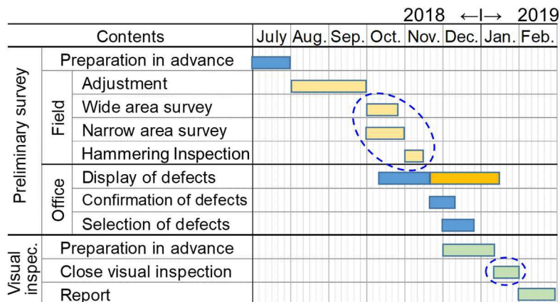
Figure 5. Inspection schedule.
